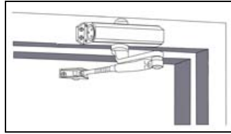
Top Jamb-Push Side
